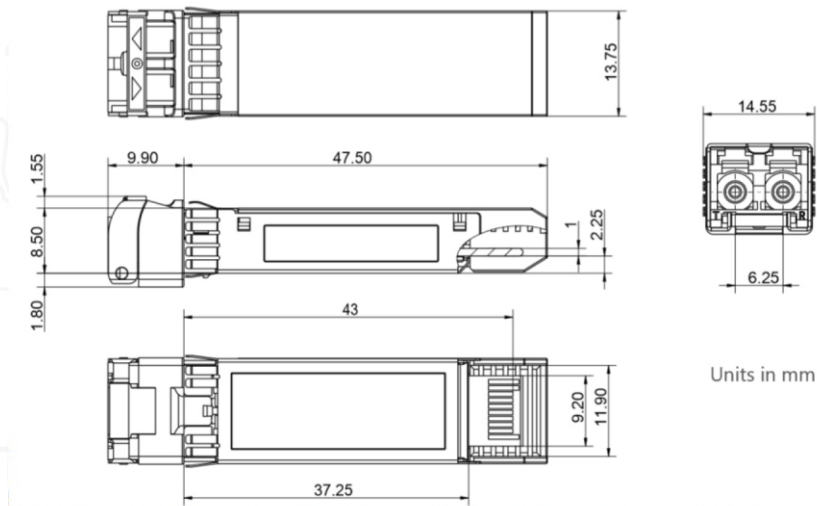
Figure2. Mechanical Outline
