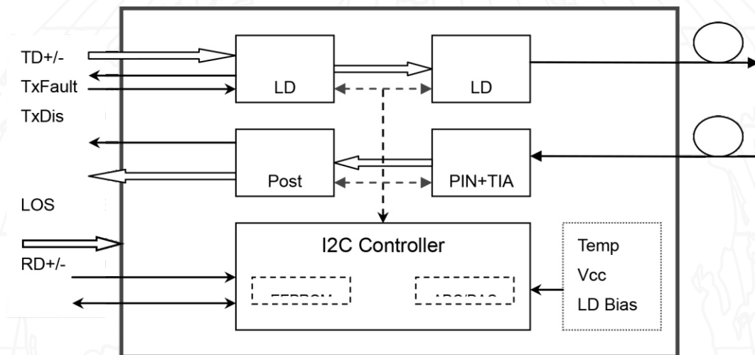
Transceiver functional diagram
